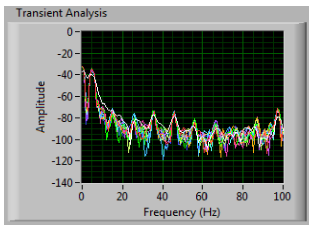
Figure 7: Transient Analysis
