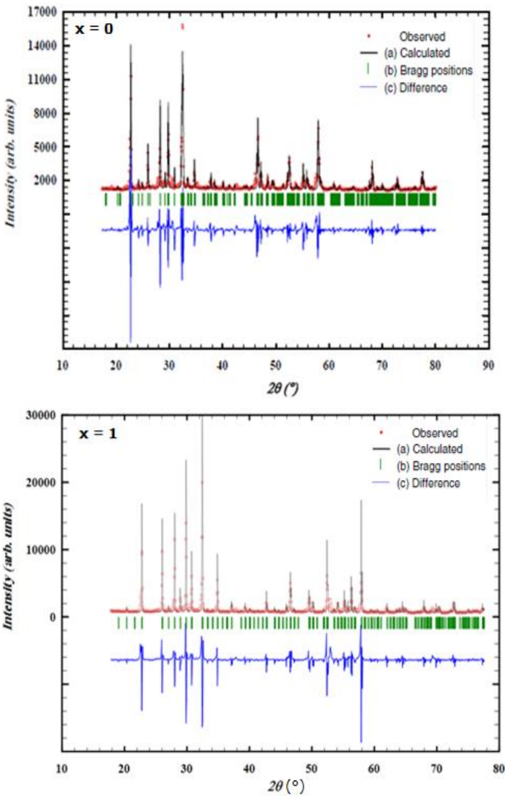
Figure 1: Observed, calculated and difference X-ray diffraction patterns for compounds with x=0 and x=1
