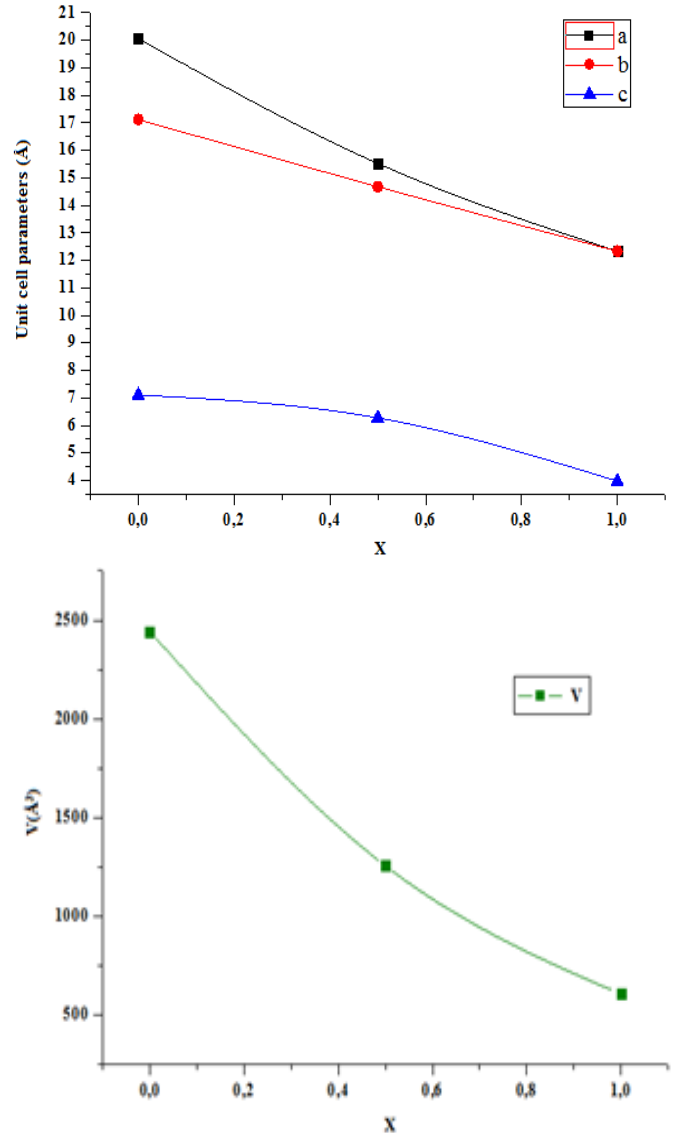
Figure 2: Evolution of the lattice parameters of Sr_{2(1-x)}Na_{(1+x)}Gd_xNb_5O_{15} as a function of the gadolinium content x .
