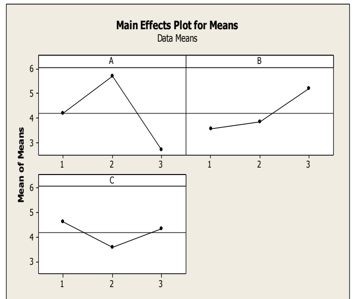
Figure 3: Effects of Process Parameters on % Elongation (Means)
