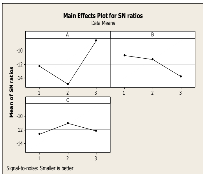
Figure 4: Effects of Process Parameters on % Elongation (S/N Ratio)
