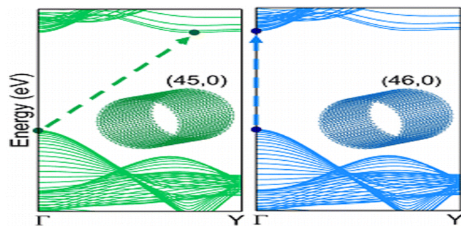
Figure 4: DFT Calculations [9]
