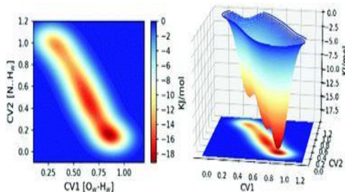
Figure 2: An in situ Meta dynamics Calculations [7]
