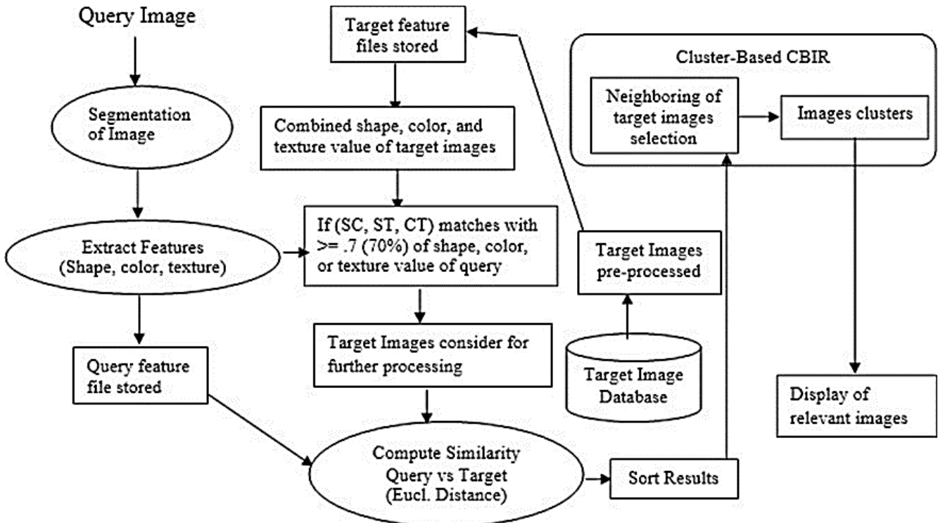
Figure 1. The CBIR System based on a fusion of visual traits
