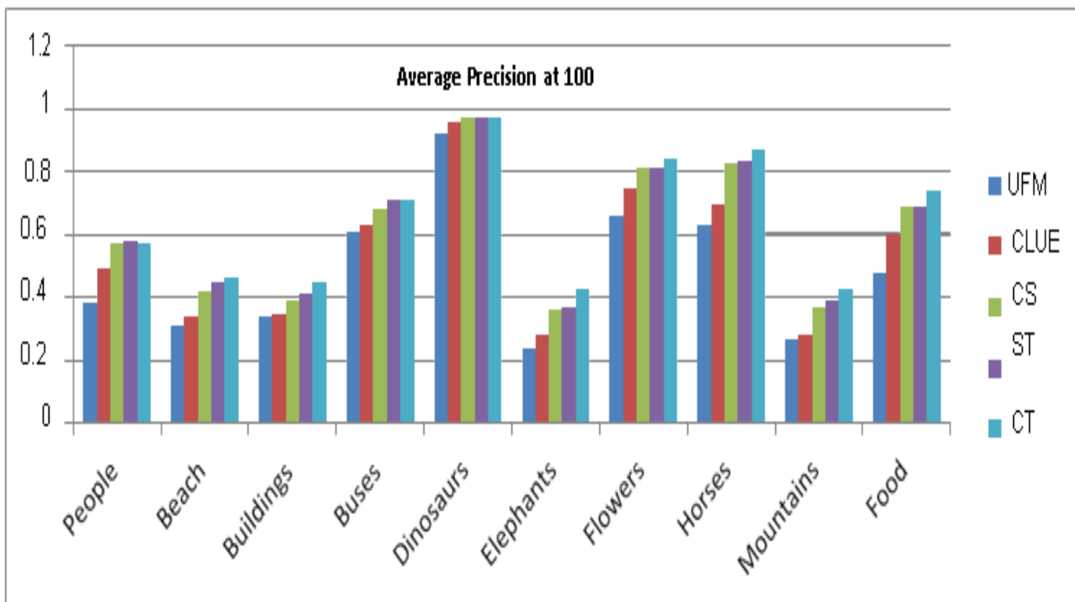
Figure 3. A comparison graph showing the average precision of five CBIR systems for each kind of image database.
